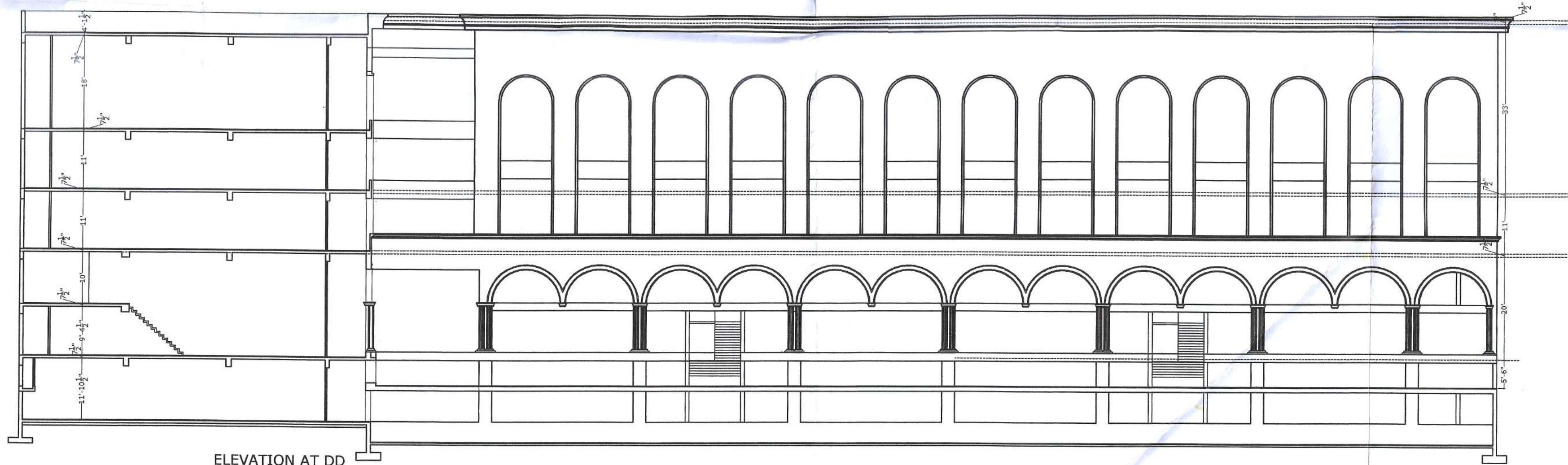
ELEVATION AT DD
