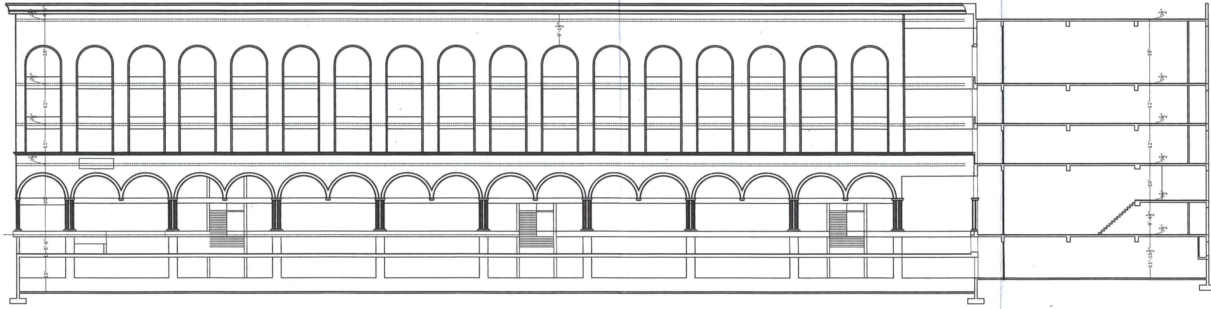
ELEVATION AT CC
