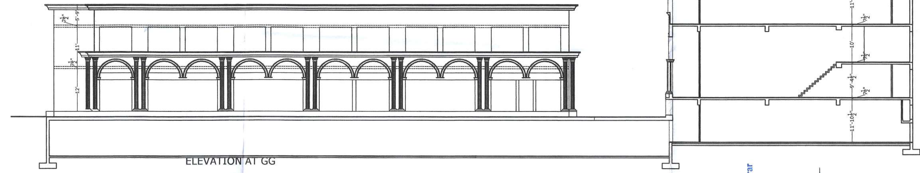
ELEVATION AT GG
